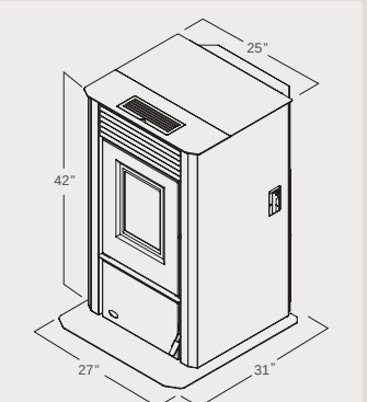
MAXX | MAXX-M Pellet Stove
