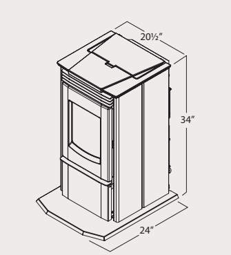
P3 Pellet Stove
