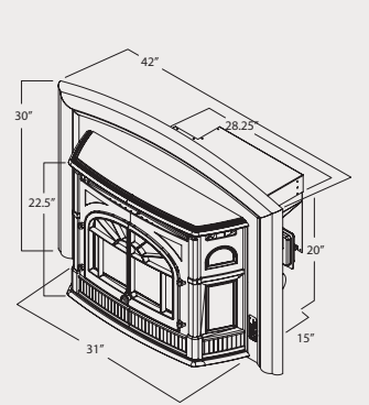
Empress Cast Iron Fireplace Insert
