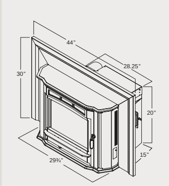
Milan Fireplace Insert
