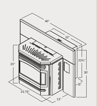
Meridian Fireplace Insert
