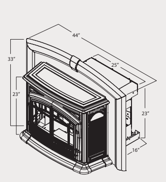
M55 Cast Iron Fireplace Insert
